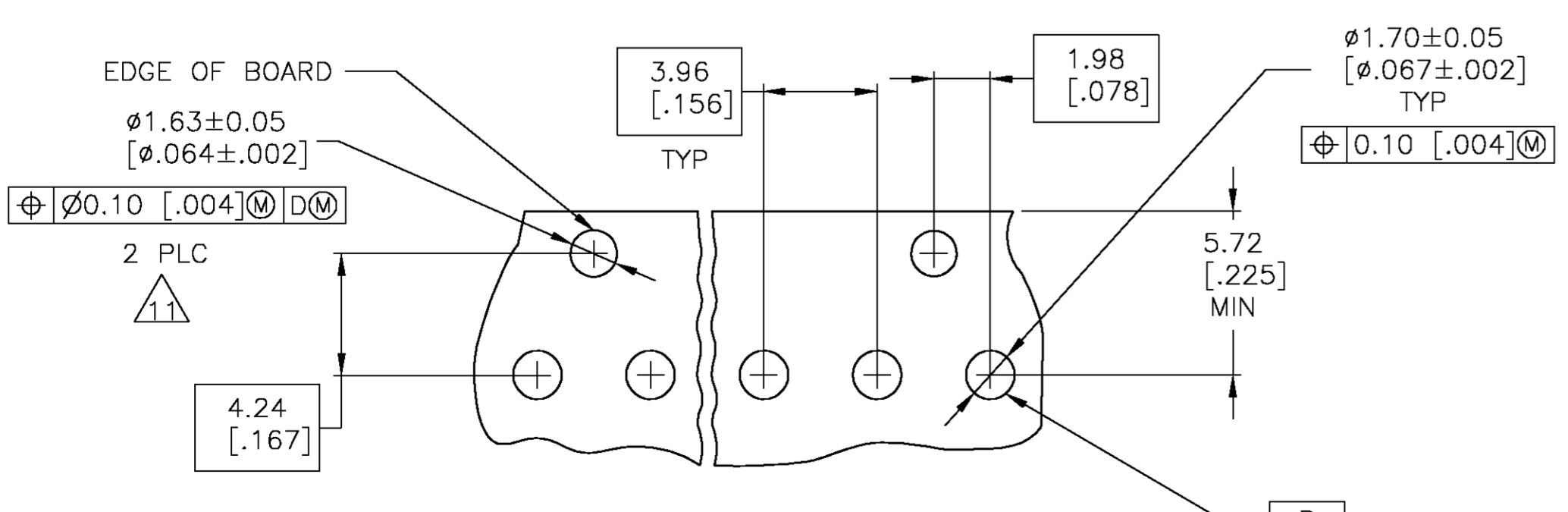
RECOMMENDED MOUNTING HOLE PATTERN FOR 1.57 [.062] THICK P.C. BOARD 2 PLC (END HOLES ONLY)
